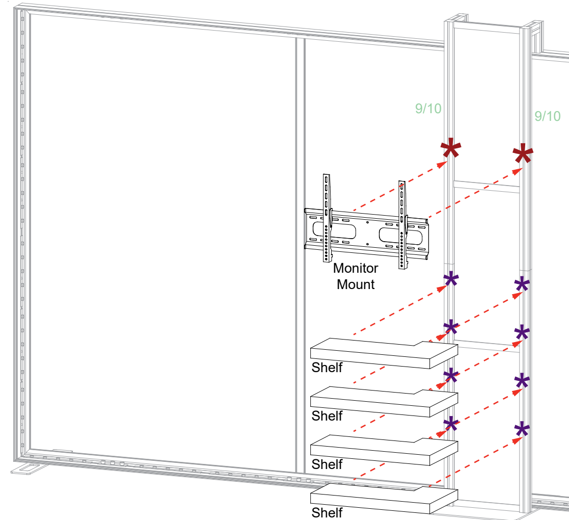
FRONT VIEW
