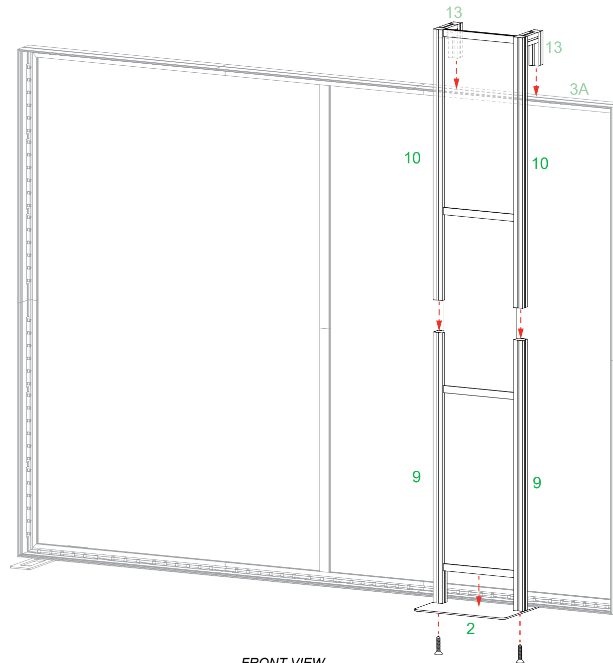
FRONT VIEW
